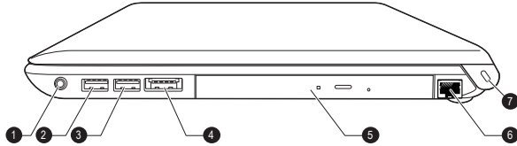
Figure 2-3 The right side of the computer (R950)
